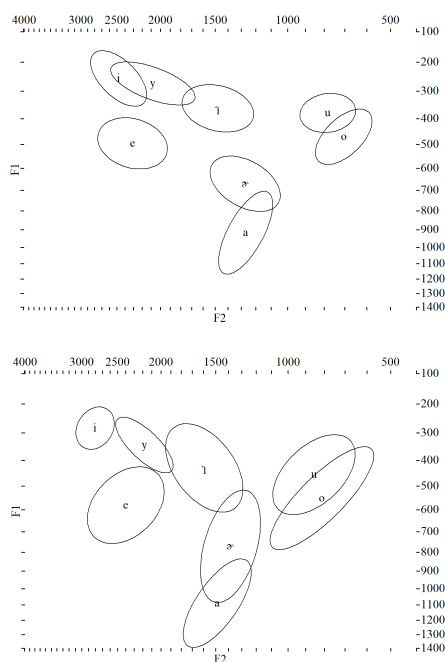
Figure 1: 2-sigma ellipses for the Chengdu monophthongs in males (upper) and females (lower).
