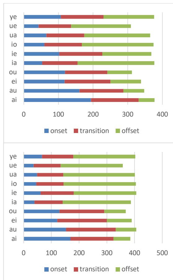
Figure 2: Temporal structure in millisecond of diphthongs in males (upper) and females (lower).
