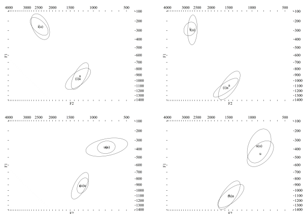
Figure 6: 2-sigma ellipses for the onset and offset of [ia ua] and corresponding monophthongs in males (left) and females (right).
