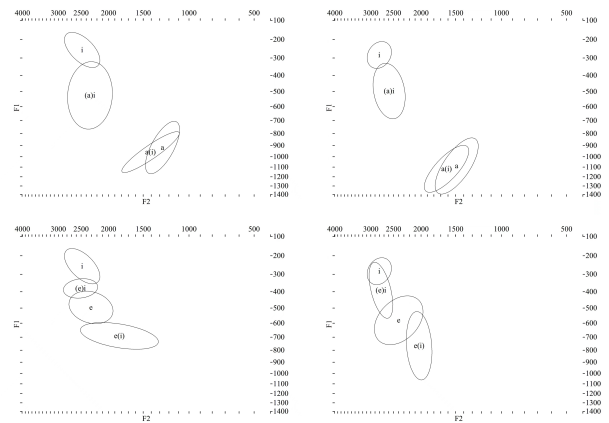
Figure 4: 2-sigma ellipses for the onset and offset of [ai ei] and corresponding monophthongs in males (left) and females (right).
