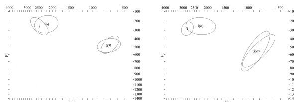
Figure 8: 2-sigma ellipses for the onset and offset of [io] and corresponding monophthongs in males (left) and females (right).
