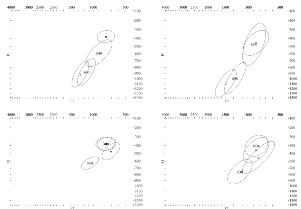
Figure 5: 2-sigma ellipses for the onset and offset of [au ou] and corresponding monophthongs in males (left) and females (right).
