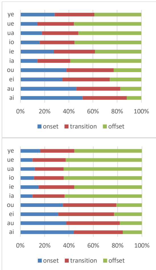
Figure 3: Temporal structure in percentage of diphthongs in males (upper) and females (lower).
