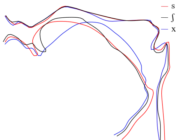
Figure 3: MRI traces of the midsagittal plane for lingual fricatives, /s/ (red), /ʃ/ (black), /x/ (blue) for US03.
